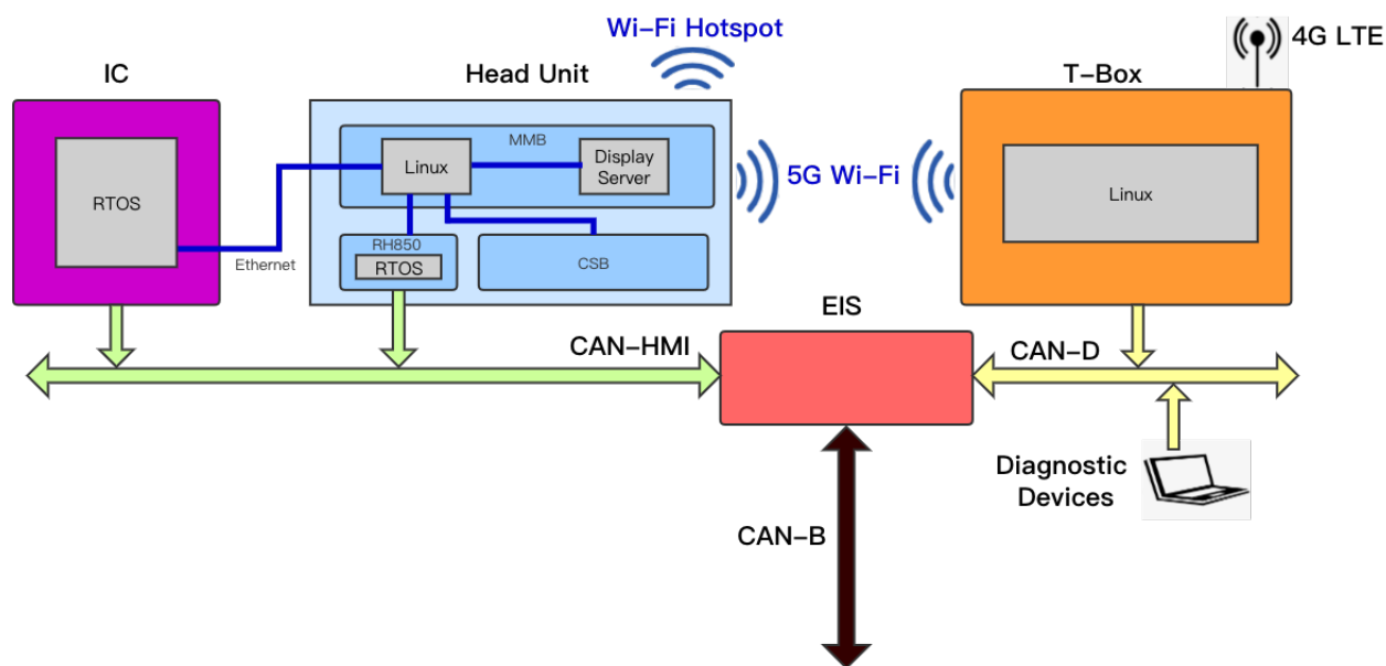
Figure 2.1: Architecture overview
