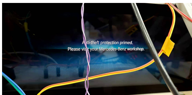
Figure 3.5: Anti-Theft screen
