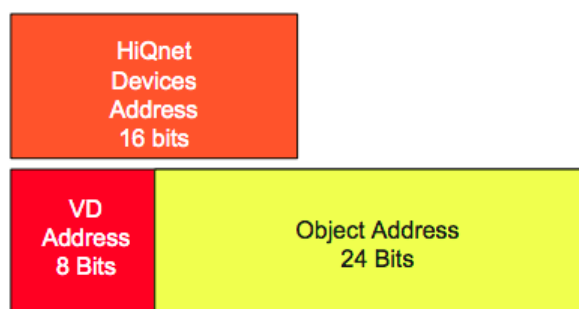
Figure 5.8: HiQnet Addressing
