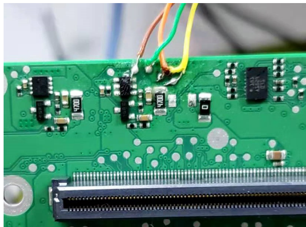
Figure 5.4: Soldered RJ45 cable to testing points
