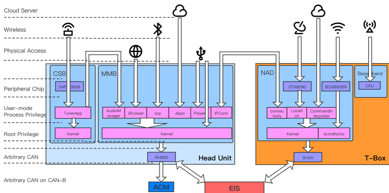
Figure 4.1: Attack surfaces
